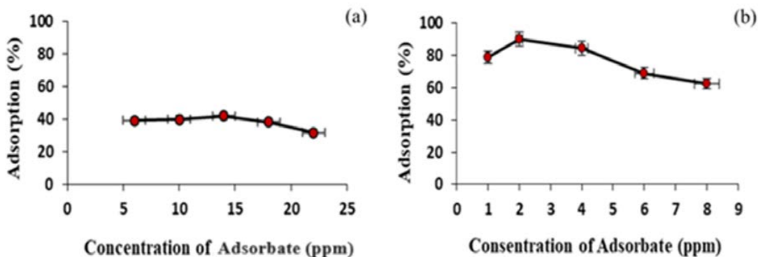
Fig. 6: Adsorption test to assess the influence of the optimal concentration of (a) ceftriaxone and (b) ciprofloxacin
