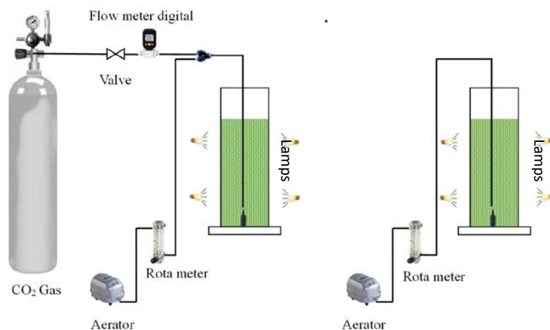
Fig. 1: Experimental photobioreactors arrangement
