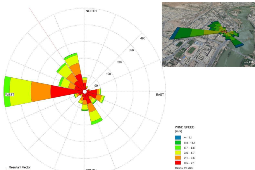
Fig. 2: Annual wind rose records obtained from Ahvaz weather station
