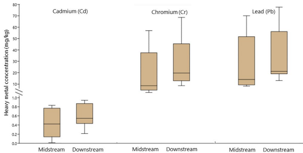
Fig. 3: Comparison of selected heavy metals concentration in midstream and downstream of Cisadane River
