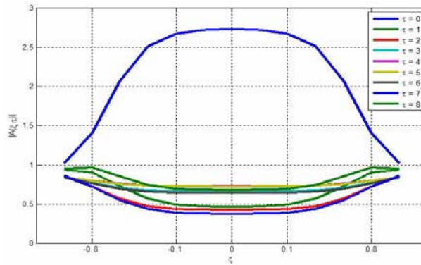
Fig. 1: Graph of envelope |A_{SFB}| for (\tilde{\tau}_0, \beta, \gamma, \tilde{\nu}) = (1, 1, 1, \sqrt{1/2}) (Fadhiliani et al., 2019)
