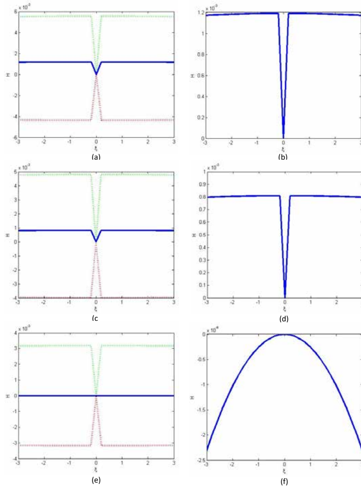
Fig. 5 : Energy distribution (left column) and Hamiltonian's curve (right column) for (\tilde{t}_0; \tilde{k}) = (0.2; 0.9186) ; (a) - (b) \tilde{\nu} = 0.5 , (c) - (d) \tilde{\nu} = 0.7 , and (e) - (f) \tilde{\nu} = 1
