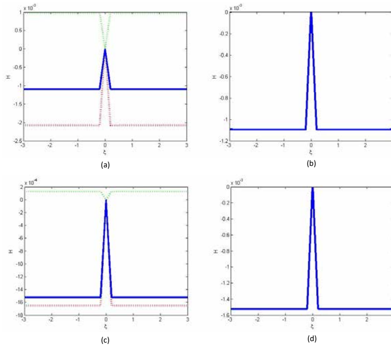
Fig. 6 : Energy distribution (left column) and Hamiltonian's curve (right column) for (\tilde{r}_0; \tilde{k}) = (0.2; 0.9186) ; (a) - (b) \tilde{\nu} = 1.3 and (c) - (d) \tilde{\nu} = 1.4
