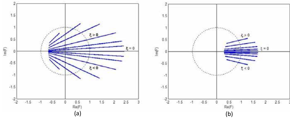
Fig. 2: Argand diagram SFB for (\tilde{\tau}_0; \tilde{k}) = (0.2; 0.9186) ; (a) \tilde{\nu} = 1 and (b) \tilde{\nu} = 1.3 (Fadhiliani et al., 2020)
