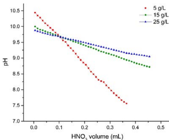
Fig. 8: Potentiometric mass titration curves of am-Zr/MgFe-LDH composite samples using 0.1 M HNO 3
