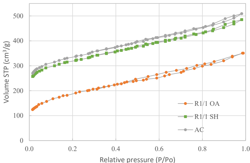
Fig. 9: N 2 adsorption-desorption isotherms of activated carbon and composites
