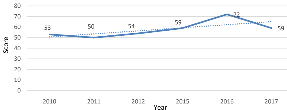
Fig. 1: Eco-IS index for Poland in selected years
